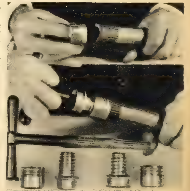
Upper view—Inserting the Couplings. Lower—The Jiffy Coupling Set and Wrench
